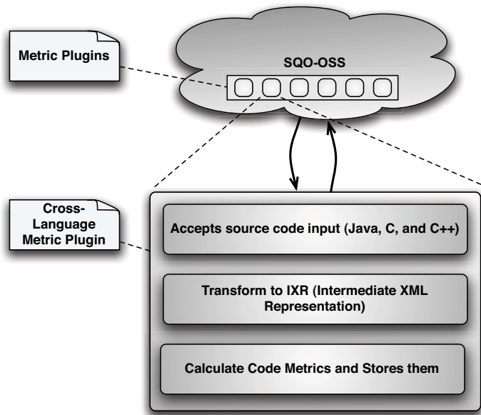
Fig. 7. The CLMT architecture
